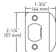
FULL LIP RADIUS STRIKE
