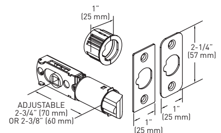
6-IN-1 ENTRY LATCH
