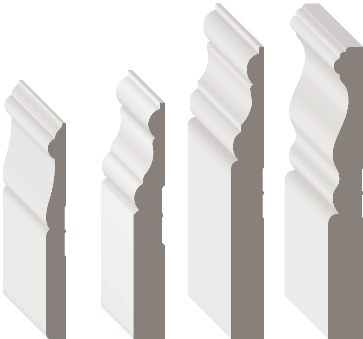
STOCK CODE MFPU8910 (1341835) DIMENSIONS \frac{3}{8} " x 3\frac{7}{8} " x 16' MDF/UL
