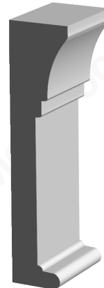
MD5060S 1-1/2" x 6-1/4"
