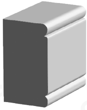
MD3322(P)T 1-1/4" x 2-1/4"
