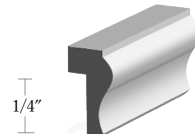
MD292M 9/16" x 1-1/8"
